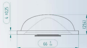
A893 6622 Beam angle 120°
