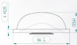
A892 6624 Beam angle 90°
